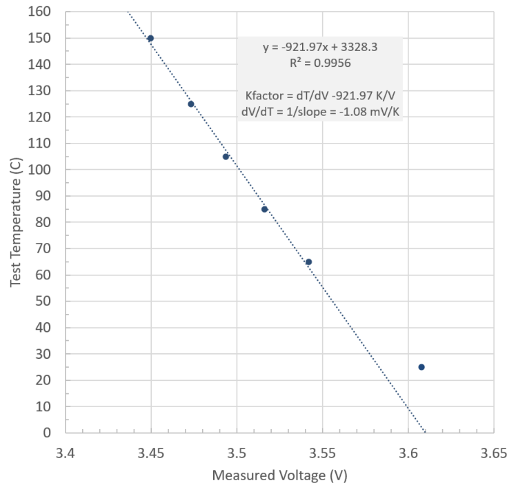
Figure 7. Illustration of K-factor calculation for a 1 mm 2 Luminus blue LED.
